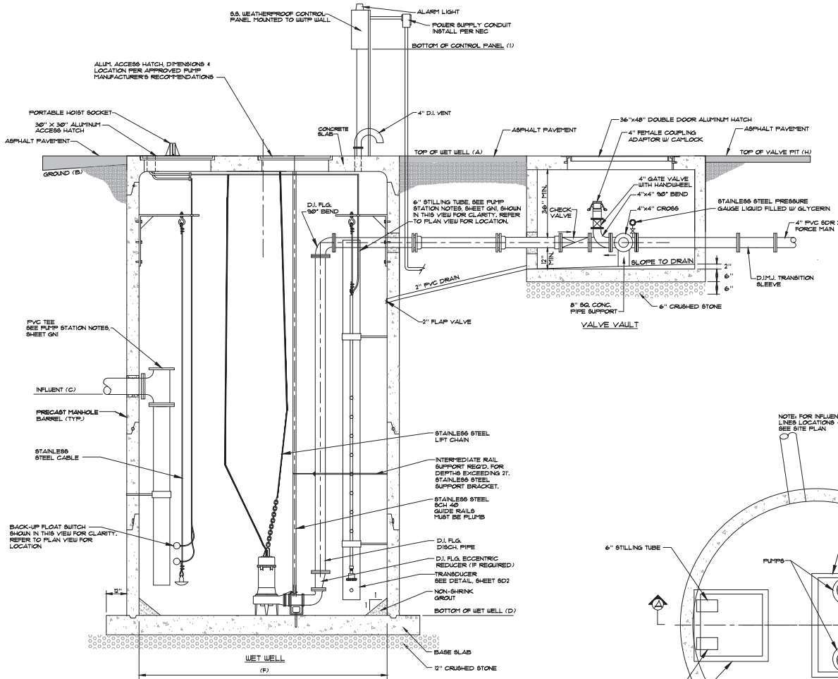
A SECTION WUTP PUMP STATION N.T.S.
