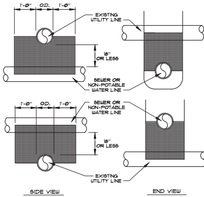
5 UTILITY CROSSING / ENCASMENT NOT TO SCALE
