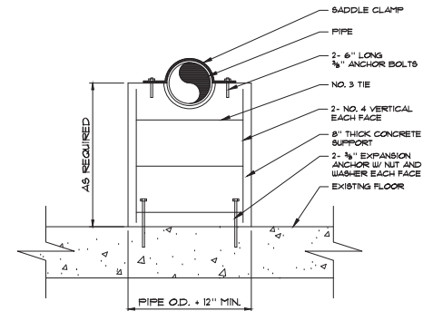
2 PIPE SUPPORT NOT TO SCALE
