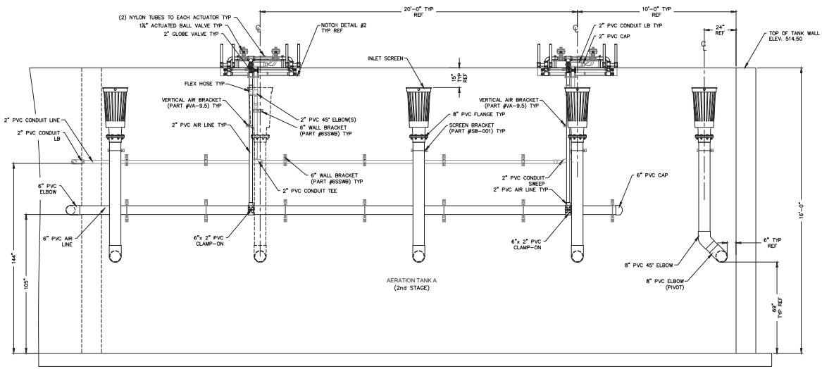
SECTION G-G
