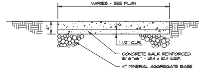
4 CONCRETE SIDEWALK NOT TO SCALE
