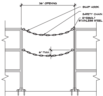
10 SAFETY CHAIN NOT TO SCALE
