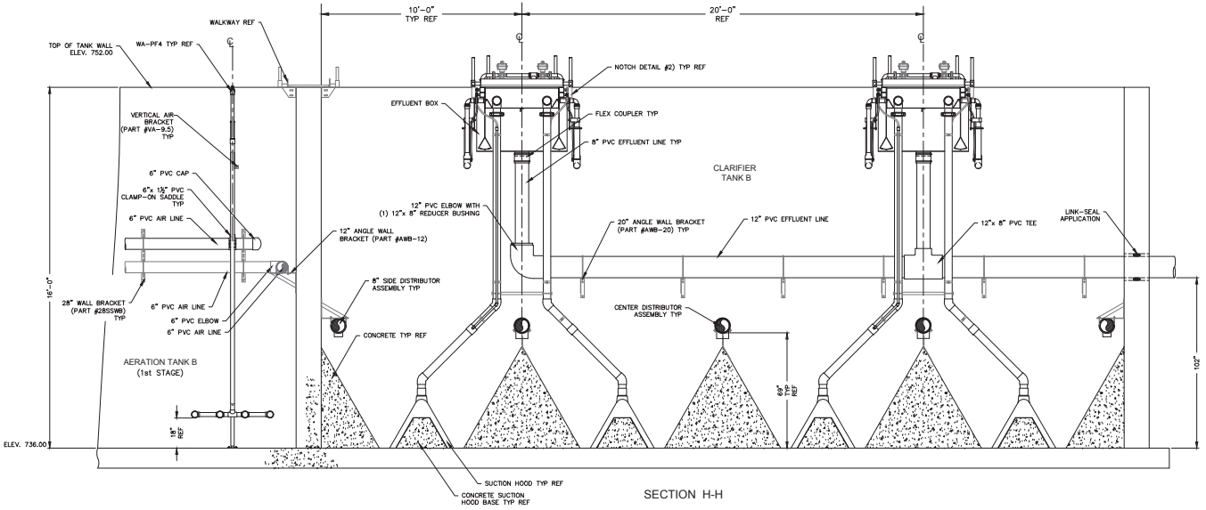
SECTION H-H
