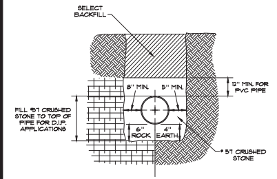
2 EMBEDMENT NOT TO SCALE
