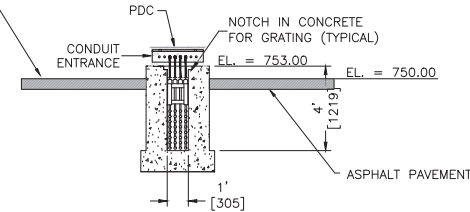
SECTION B
