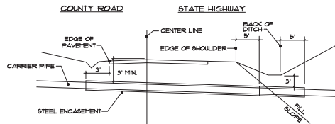
8 TYPICAL ROAD CROSSING NOT TO SCALE
