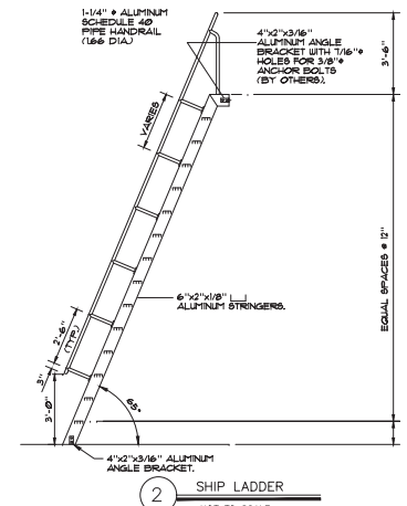
2 SHIP LADDER NOT TO SCALE
