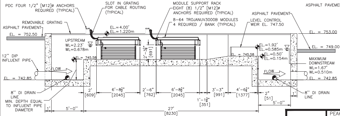
SECTION A
