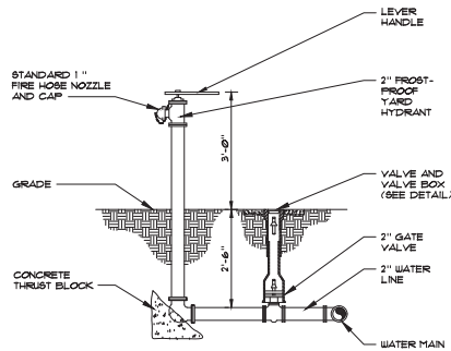
6 1" YARD HYDRANT NOT TO SCALE
