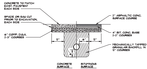
7 PAVEMENT REPAIR NOT TO SCALE
