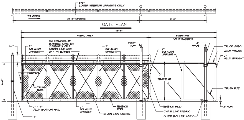
32'-0" SINGLE CANTILEVERED SLIDING GATE N.T.S.
