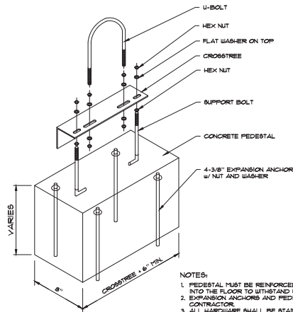
3 CONCRETE SUPPORT NOT TO SCALE
