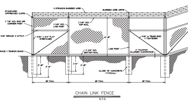
3 FENCE NOT TO SCALE
