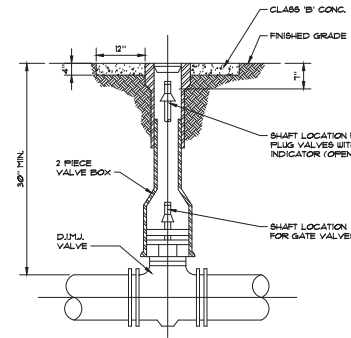
3 VALVE AND VALVE BOX NOT TO SCALE
