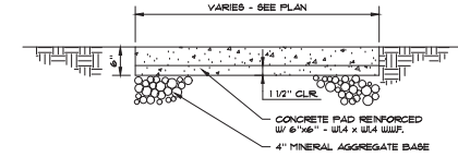
2 EQUIPMENT PAD NOT TO SCALE
