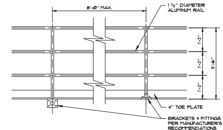
3 HANDRAIL NOT TO SCALE
