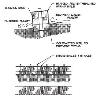
5 EROSION CONTROL NOT TO SCALE
