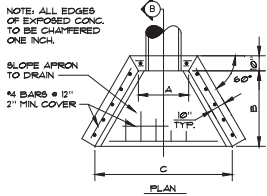
9 HEADWALL/ENDWALL NOT TO SCALE
