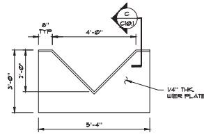
SHARP CRESTED ALUMINUM WEIR PLATE - 90° V-NOTCH SCALE: 1/2" = 1'-0"
