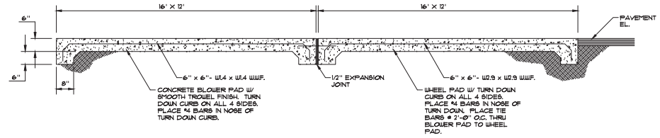
1 BLOWER PAD NOT TO SCALE
